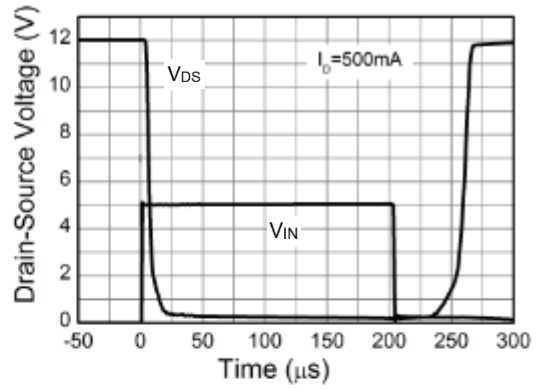
Switching Speed
