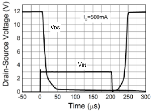
Switching Speed
