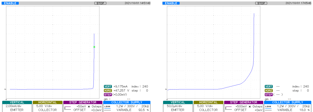
Figure 7. Typical V_{DS} Clamp Characteristic
