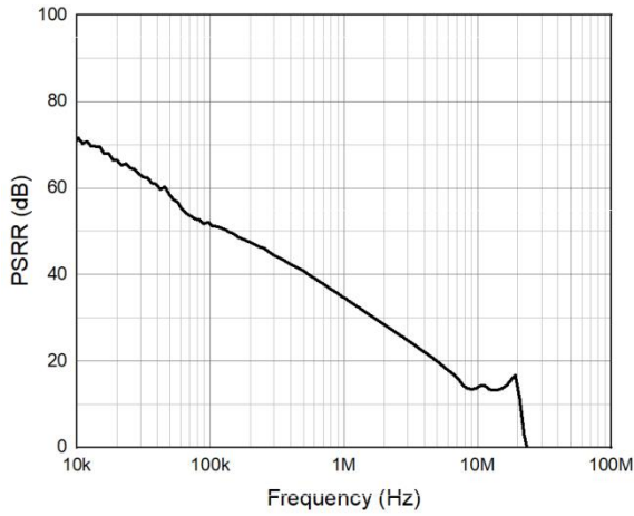
Figure 7. PSRR vs. frequency V_S = 5\text{ V}, A_V = +1
