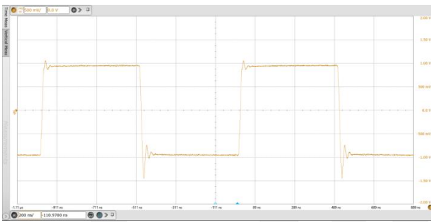
Figure 11. Large signal step response V_S = 10\text{ V}, V_{OUT} = 2\text{ V}_{PP}
