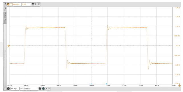
Figure 12. Large signal step response V_S = 10\text{ V}, V_{OUT} = 2\text{ V}_{PP}, G = -1
