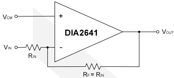
Figure 13. Typical application: gain = -1
