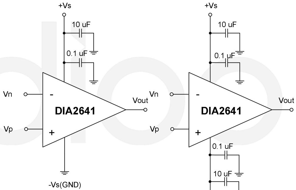
Figure 15. Amplifier with bypass capacitors
