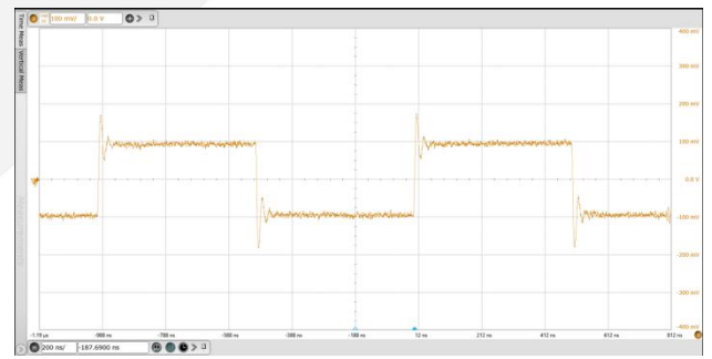
Figure 10. Small signal step response V_S = 10\text{ V}, V_{OUT} = 0.2\text{ V}_{PP}, G = 2
