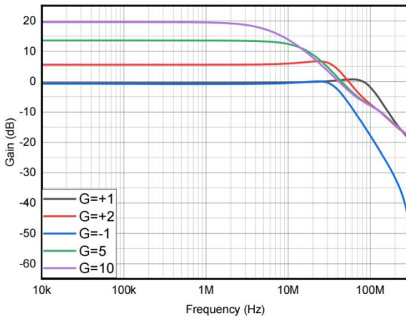
Figure 3. Closed loop gain vs. frequency for various gain
