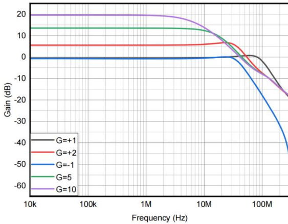
Figure 1. Closed loop gain vs. frequency for various gain
