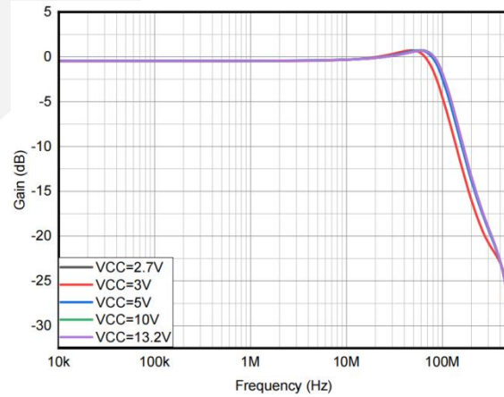
Figure 4. Closed loop frequency response for various supplies
