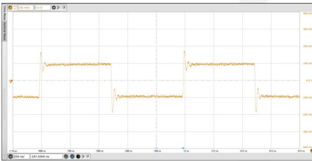
Figure 9. Small signal step response V_S = 3\text{ V}, V_{OUT} = 0.2\text{ V}_{PP}, G = 2
