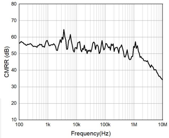
Figure 8. CMRR vs. frequency V_S = 5\text{ V}, A_V = +2
