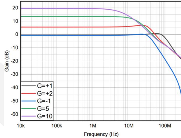
Figure 2. Closed loop gain vs. frequency for various gain
