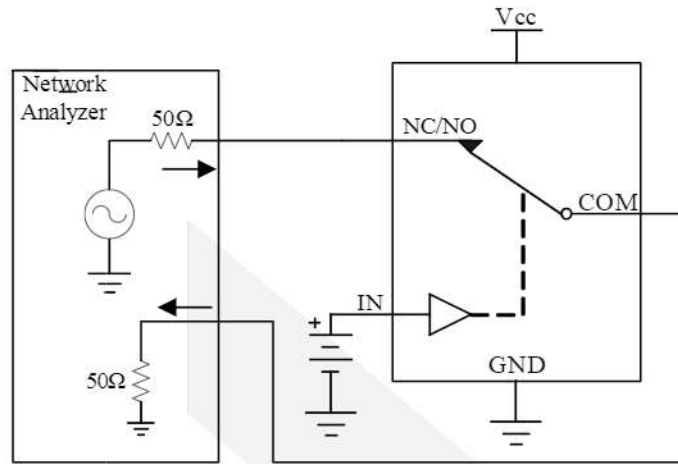
Figure 5 Bandwidth
