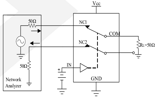
Figure 6 Channel-to-channel crosstalk
