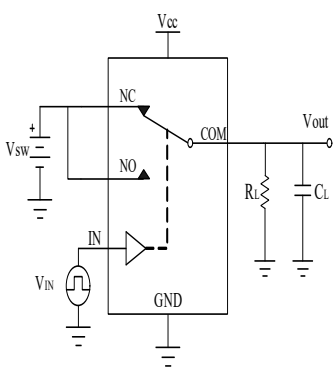
Figure 8 Break-Before-Make
