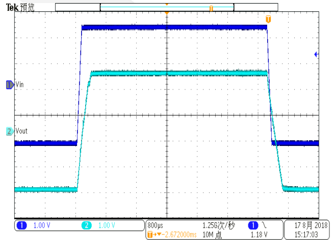
Large-Signal Response
