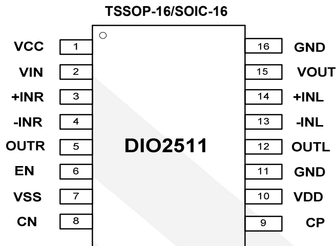
Figure 1 Pin Assignment
