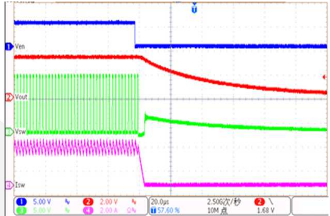
Shut down from Enable ( V_{IN}=12V, V_{OUT}=3.3V, Load=1\Omega )
