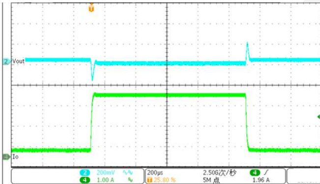
Load transient ( V_{IN}=12V, V_{OUT}=3.3V, Load=0.3-3A )
