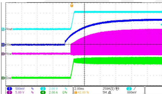
Start up from V_{IN}
