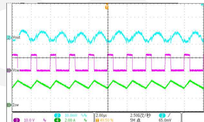
Ripple ( V_{IN}=12V, V_{OUT}=3.3V, Load=3A )
