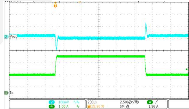
Load transient ( V_{IN}=12V, V_{OUT}=3.3V, Load=1.5-3A )
