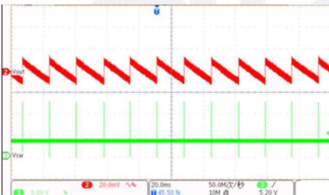
Ripple ( V_{IN}=12V, V_{OUT}=3.3V, Load=0A )
