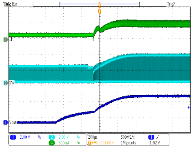
Short Circuit Recovery Vin=1.2V Vout=3.3V short -> Load=22Ω
