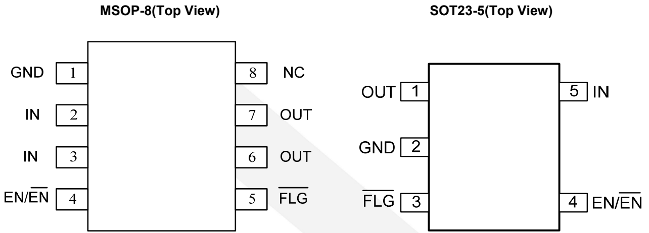
Figure 1 Pin Assignment
