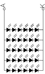
Circuit Diagram(LED SMT 6*5=30 PCS), Color: WHITE Vf=18V, If=300ma Brightness 1000cd/m² (TIP)
