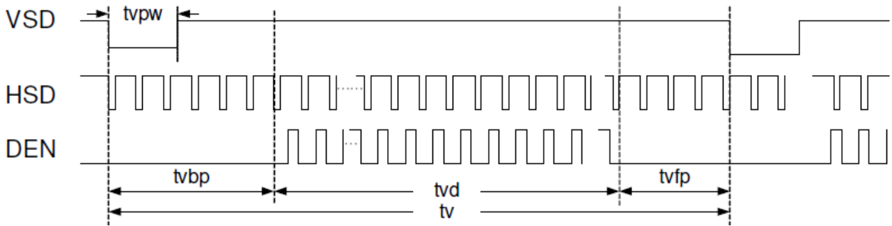
Figure: Vertical input timing diagram
