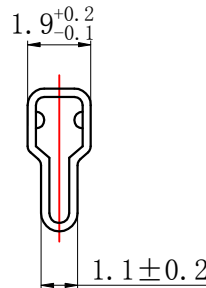
SECTION C-C
