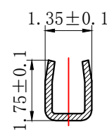
SECTION C-C
