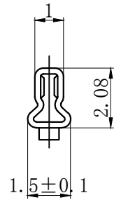
SECTION C-C
