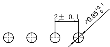
PCB LAYOUT
