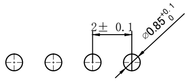
PCB LAYOUT
