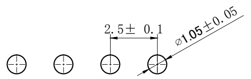
PCB LAYOUT
