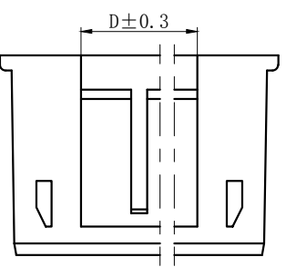
4-5PIN
