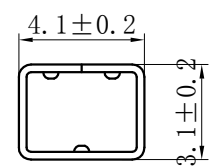
SECTION C-C
