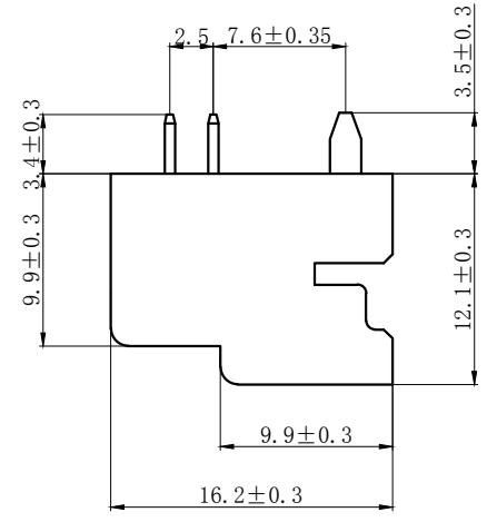
18-40PIN
