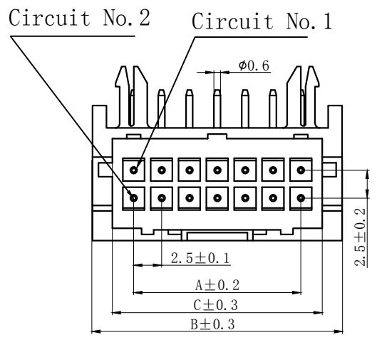
4-16PIN
