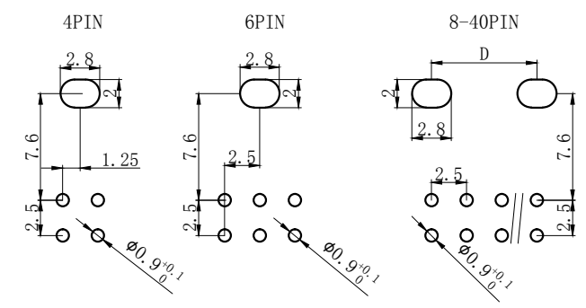
PCB LAYOUT
