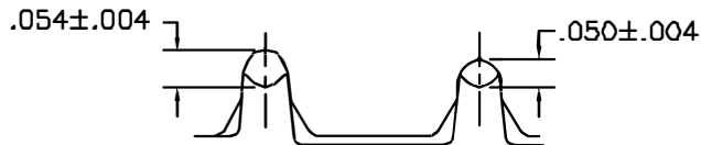
INSULATION CRIMP JAWS GMT225 -1 & -3
