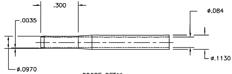
PROBE DETAIL
