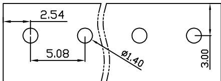
PCB Layout
