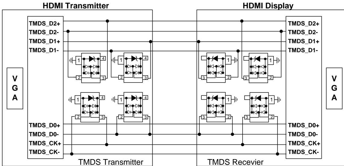
PRTR5V0U2X-N on HDMI Port Application
