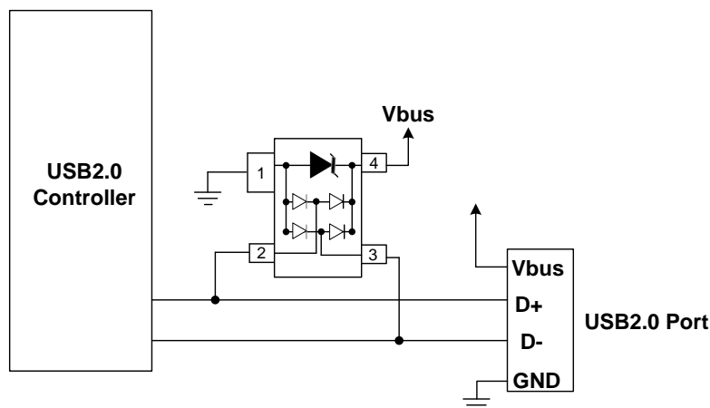
PRTR5V0U2X-N on USB2.0 Port Application
