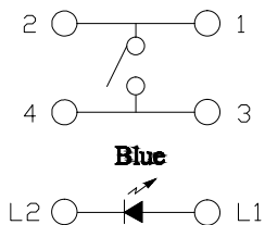
ELECTRICAL DIAGRAM
