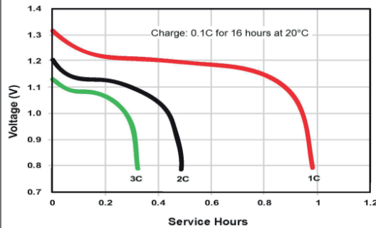
High Rate Discharge
