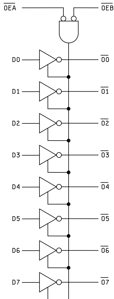
FIGURE 3. Logic diagram.
