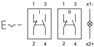
9 Illuminated pushbutton actuator page 6
