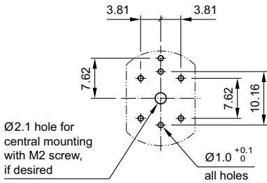
Terminals (rearside)
