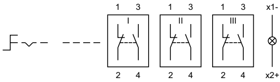
22 Selector switch 2 positions page 11
