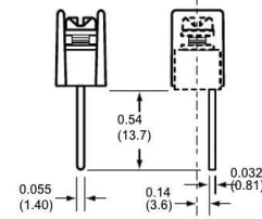
07 Extended Pin
