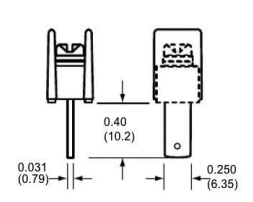
09 0.250" QC short
