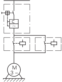
Complete devices PKZ and DILM on BBA for reversing starters
