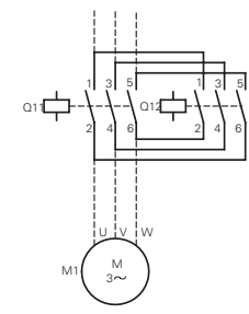
DIULM7/21 to DIULM65/11 with mechanical interlock
