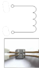
Figure 1. DCR test
