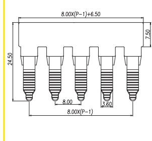
Dimensions - mm
