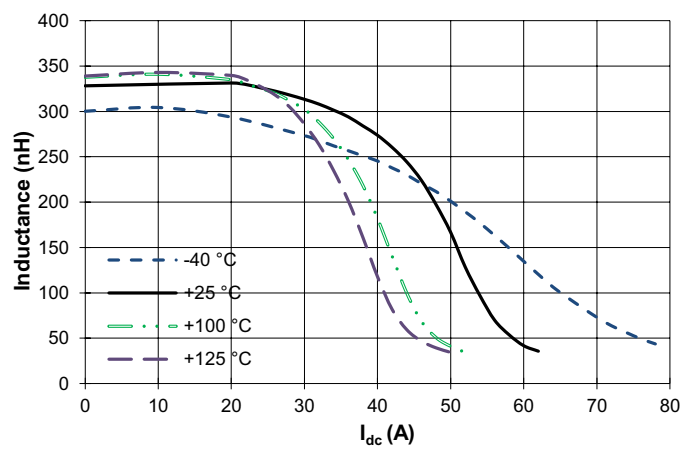
FP1010V5-R330-R
