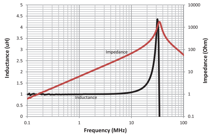
HCM1A1307V2-1R0-R
