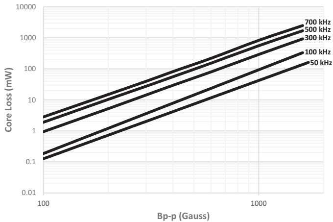
HCM1A1307V2-3R3-R
