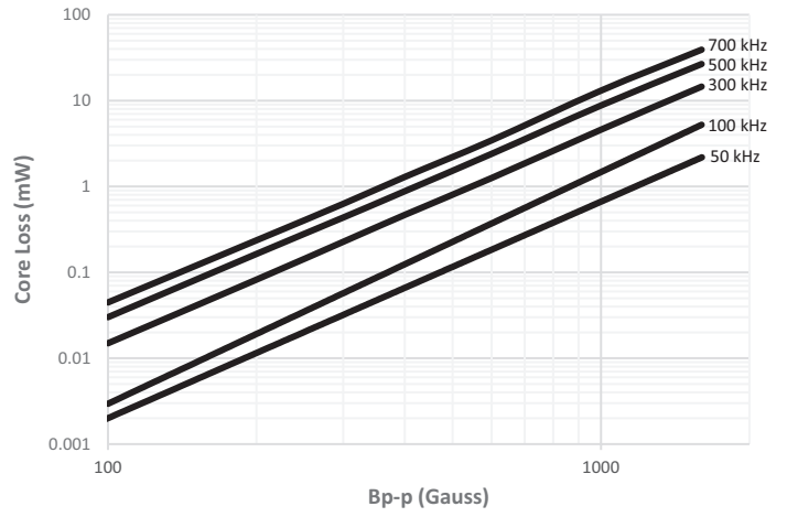
HCM1A4020V2-R68-R
