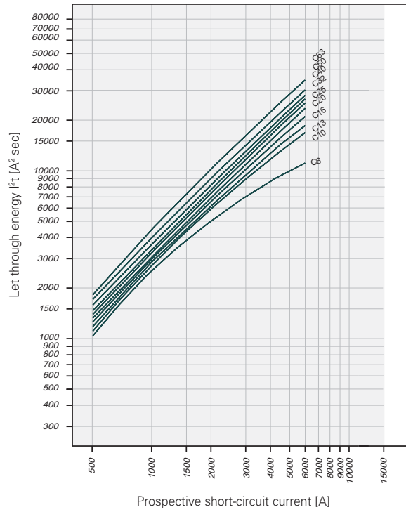
Let-through Energy HN, Characteristic C, 1-pole
