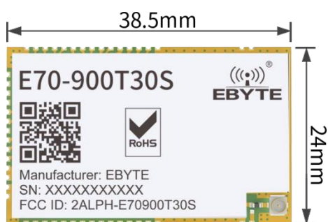
图 1: E70-900T30S
