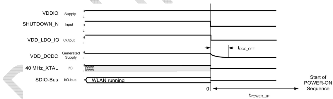
Figure 11: Shutdown Sequence
