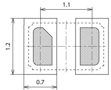
Figure 2) Suggested Land Pattern
