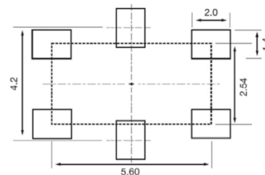
Figure 2) Land Pattern
