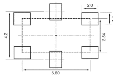
Figure 2) Land Pattern
