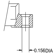
VARIATION 04 .156 +0.002 -0.000 DIA. MOUNTING HOLE
