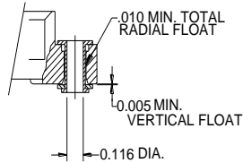
VARIATION 03 .116 +0.003 -0.000 I.D. FLOATING EYELET
