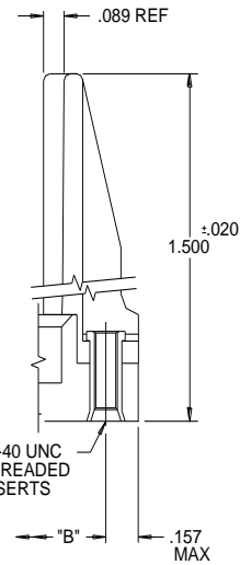
MOUNTING OPTION CODE #78
