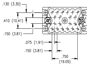
20 PIN PLUG
