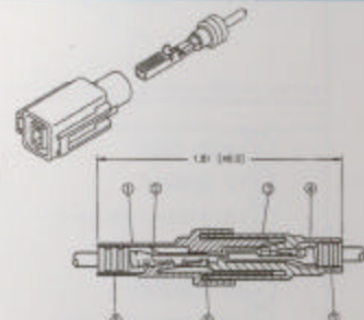
① 568-001-000-200 ② U TERMINAL ③ 568-001-000-100 ④ F TERMINAL ⑤ WIRE SEAL ⑥ HOUSING SEAL
