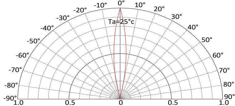
Radiation Pattern
